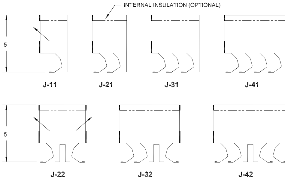
END BRACKET DETAIL
