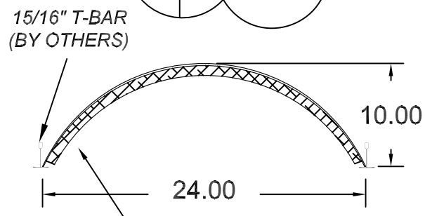
OPTIONAL INSULATION (SHOWN FOR REFERENCE ONLY)
